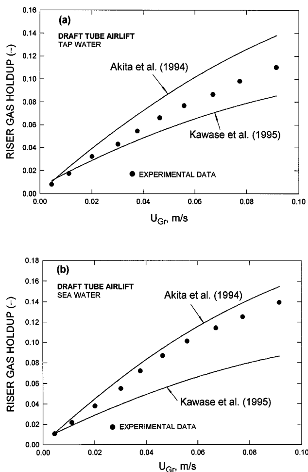
Figure 4. Comparison of the measured riser gas holdup in the draft-tube airlift vessel with published data: (a) tap water; (b) sea- or saltwater.
