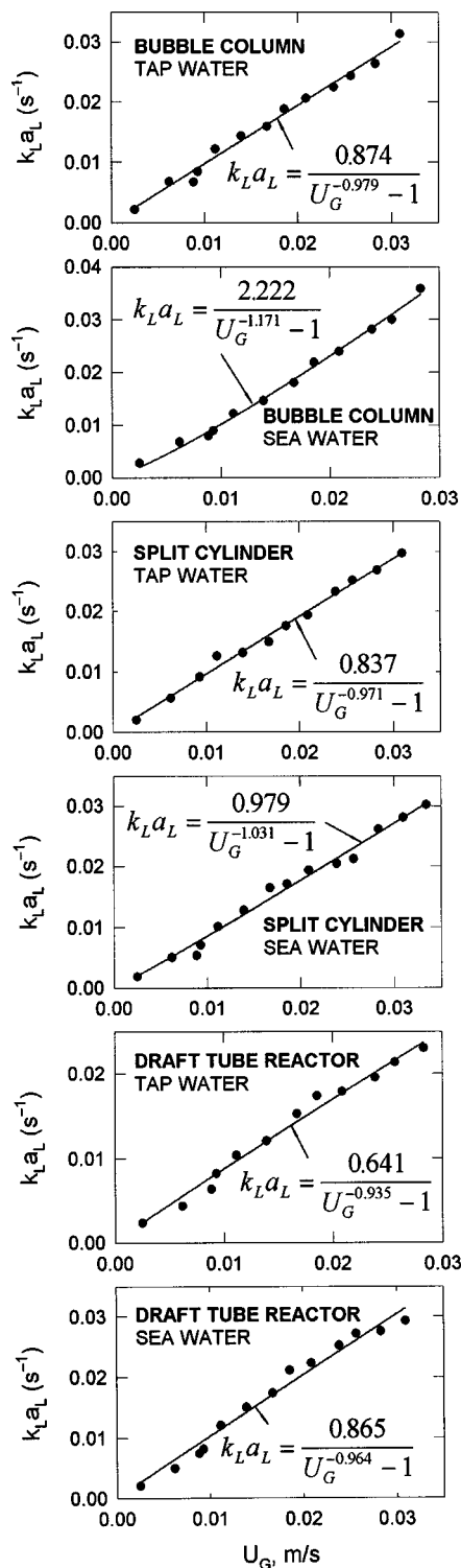
Figure 12. Correlation of the measured k_L a_L with the superficial aeration velocity U_G according to Eq. 10 or Eq. 13; data are shown for all reactor-fluid combinations.
