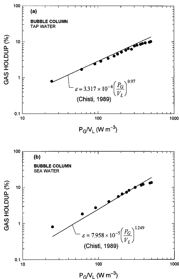
Figure 3. Comparison of the measured gas holdup in the bubble column with the correlations of Chisti (1989): (a) tap water; (b) sea- or saltwater.
