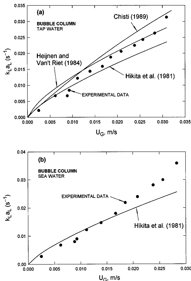
Figure 11. Comparison of the measured k_L a_L in bubble column with the published correlations: (a) tap water; (b) sea- or saltwater.
